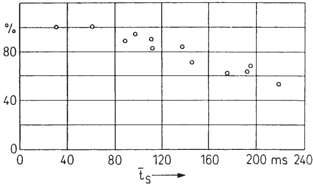
Figure 7.14 Relation between speech intelligibility and centre time t_s (after Kürer 18 ).
