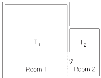
Figure 9.7 Coupled rooms.
