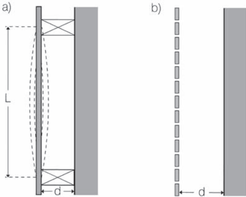
Figure 6.3 Resonance absorbers: (a) with vibrating panel; (b) with perforated panel.
