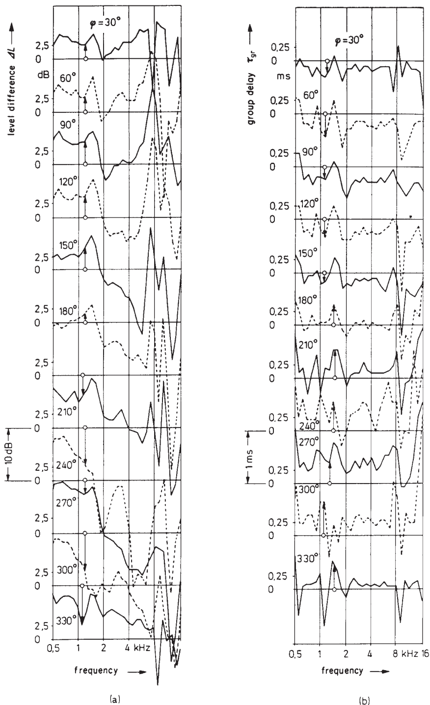
Figure 1.6 Head transfer functions for several directions of sound incidence in the horizontal plane, relative to that for frontal incidence, average over 25 subjects: (a) amplitude (in logarithmic representation); (b) group delay (after Blauert 3 ).
