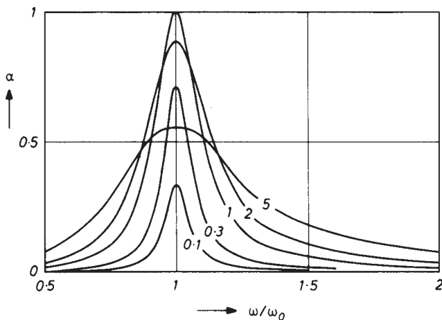
Figure 6.4 Absorption coefficient \alpha (calculated) of resonance absorbers, similar to Fig. 6.3, as a function of frequency for normal sound incidence and for M\omega_0 = 10\rho_0c . Parameter is the ratio r_s/\rho_0c .
