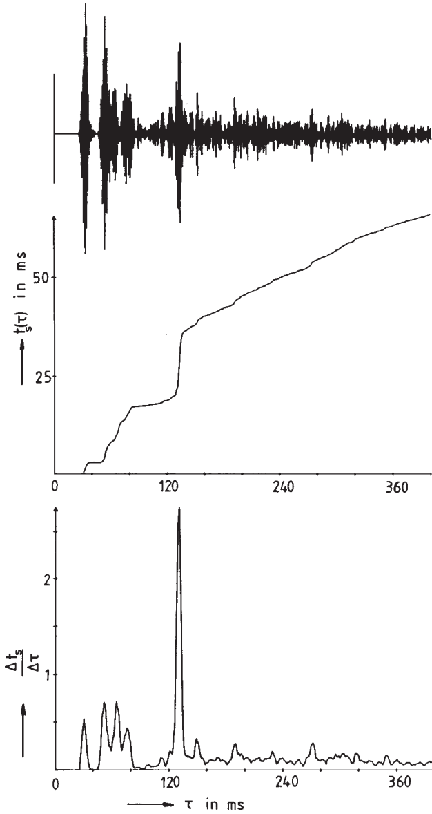
Figure 7.12 First 400 ms of a room impulse response, of the associated build-up function t_s(\tau) and of the difference quotient \Delta t_s(\tau)/\Delta \tau (with \Delta \tau = 5 ms). EC is 2.75 in this example.
