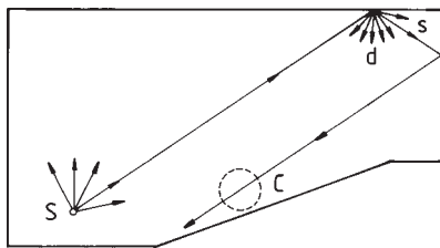
Figure 9.10 Principle of digital ray tracing. S = sound source, C = counting sphere, s = specular reflection and d = diffuse reflection.
