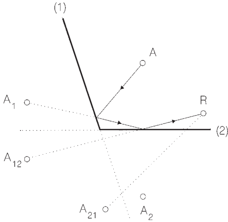
Figure 9.13 Valid and invalid image sources. Image source A_{21} is invalid, i.e. ‘invisible’ from the given receiver R.
