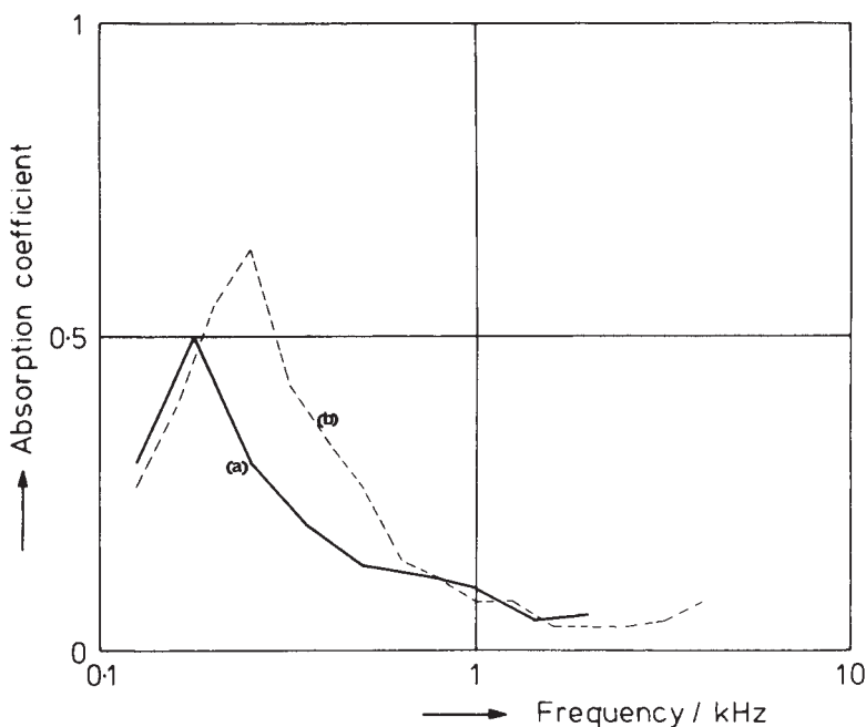
Figure 6.5 Measured absorption coefficient of resonance absorbers at random sound incidence: (a) wooden panels, 8 mm thick, 5 \text{ kg/m}^2 , 30 mm distant from rigid wall, with 20 mm thick rock wool plate behind ( 33.2 \text{ Rayl/cm} ); (b) panels, 9.5 mm thick, perforated at 1.6% (diameter of holes 6 mm), 5 cm distant from wall, air space filled with glass wool.
