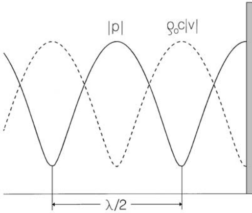
Figure 2.3 Standing sound wave in front of a plane surface with real reflection factor R = 0.7 . — magnitude of sound pressure; - - - magnitude of particle velocity.
