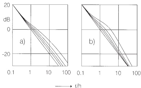
Figure 9.9 Sound pressure level in an infinite flat room as a function of distance r divided by the room height b . The absorption coefficient \alpha of the walls is (from bottom to top): 1, 0.7, 0.5, 0.3, and 0.1. (a) smooth walls; (b) diffusely reflecting walls.
