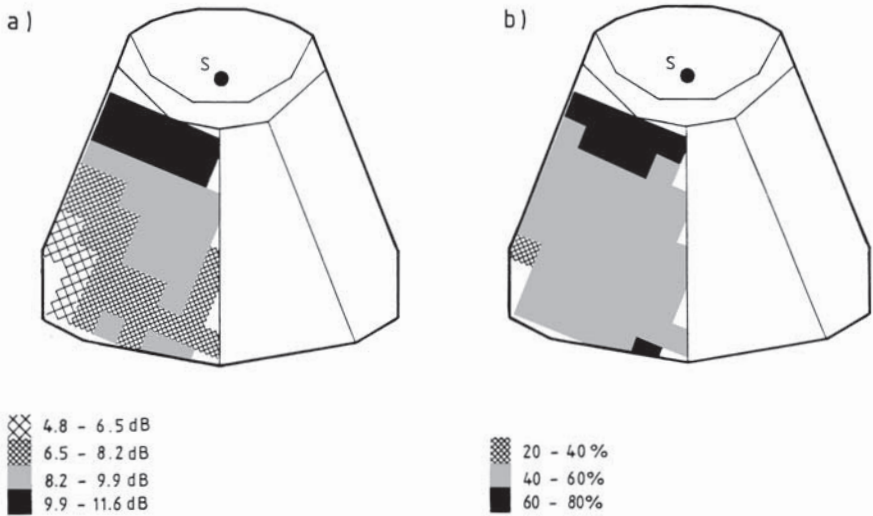
Figure 9.12 Distribution (a) of the stationary sound pressure level and (b) of the 'definition' in a large lecture hall (after Vorländer 16 ).
