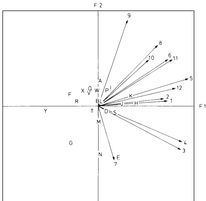
Figure 7.19 Individual preference scales of 12 test subjects (arrows) and 22 concert hall points (A, B, . . . , Y) represented in the F_1 - F_2 plane of a four-dimensional perceptual space.
