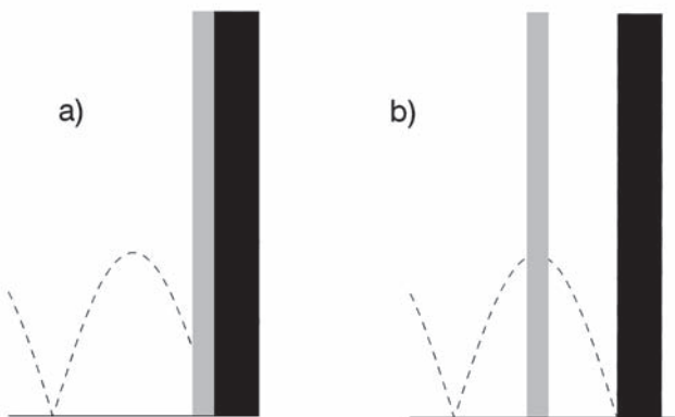
Figure 6.12 Porous layer in front of a rigid wall (dotted line: distribution of particle velocity without layer: (a) layer immediately on the wall; (b) layer at some distance from the wall.
